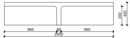
Back view
